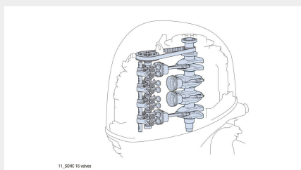
11. SOHC 16 valves
